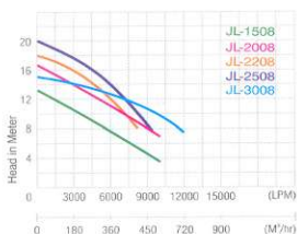
Family Performance Curve
