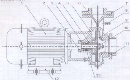
Gland Packing Arrangement
