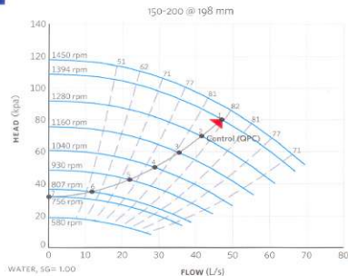
FIGURE 2 - System control curve
