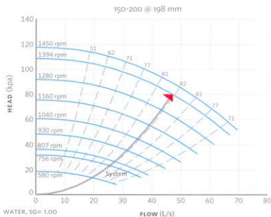
FIGURE 4 - Constant curve control
