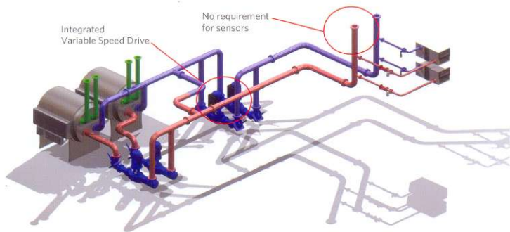
FIGURE 3 - Primary/secondary chilled or heating water system incorporating Armstrong ivs sensorless pumps
