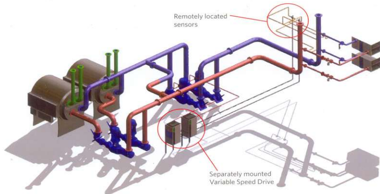
FIGURE 1 - Typical primary/secondary chilled or heating water system incorporating Variable Speed Drives
